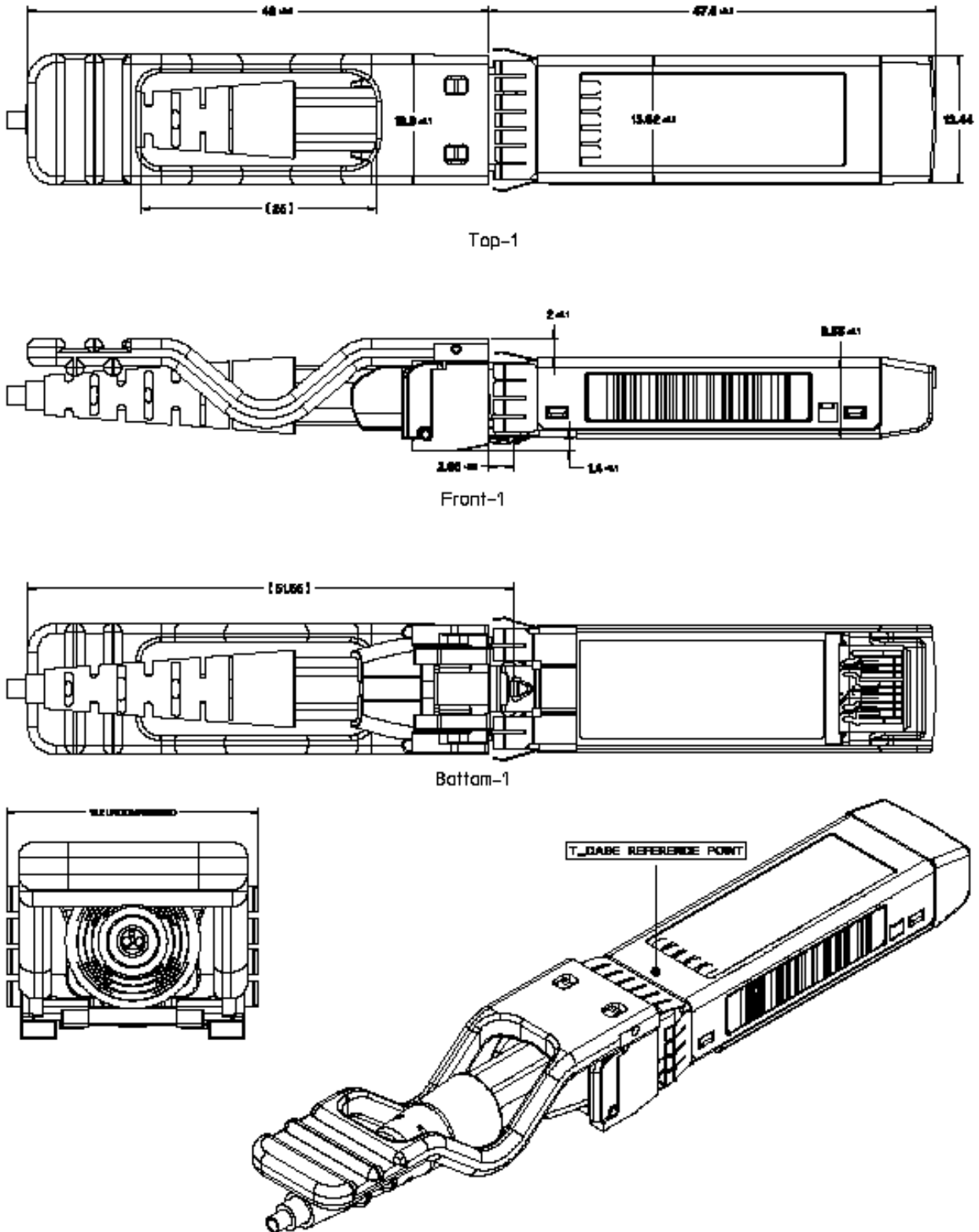
Figure 4. Module drawing
