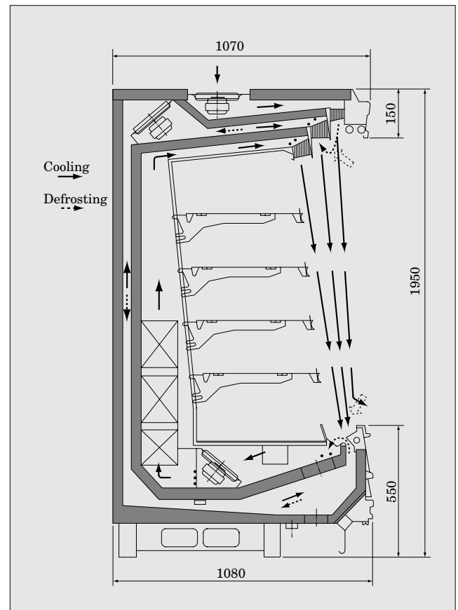
Fig. 3 Structure of the conventional device
