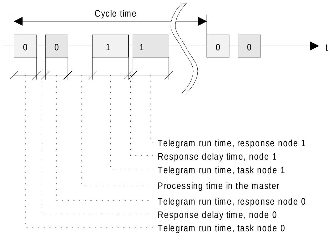
Fig. 5.2: Cycle time
