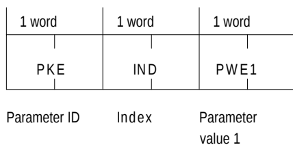
Fig. 4.1: Structure of the PKW area 3 words
