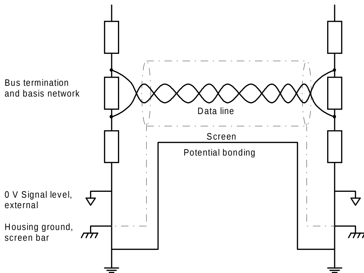
Fig. 4.2: Screening and potential bonding
