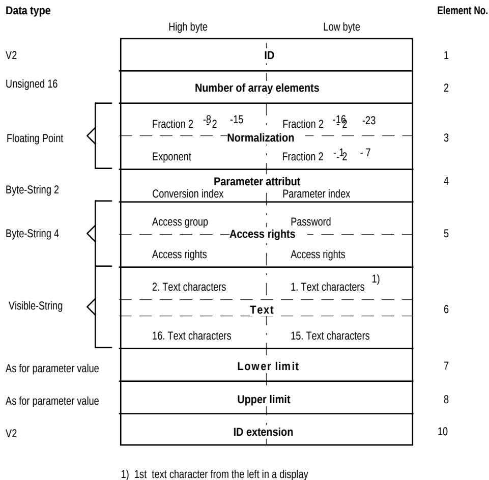
Fig. 6.1: Complete parameter description structure in the "internal memory" for SIMOVERT master drives
