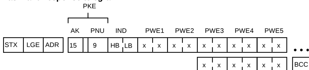
Fig. 8.9: Telegram structure to example 8
