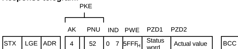
Fig. 8.4: Telegram structure to example 4
