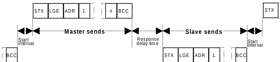
Fig. 5.3: Send sequence
