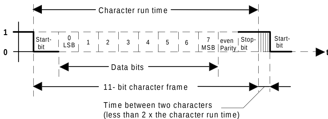
Fig. 3.2: Character frame
