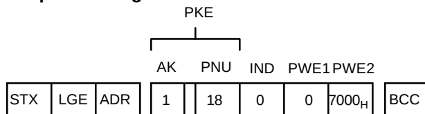
Fig. 8.6: Telegram structure to example 6
