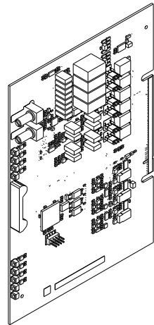
Figure 1 VCC2002-A1 Voice I/O Card
