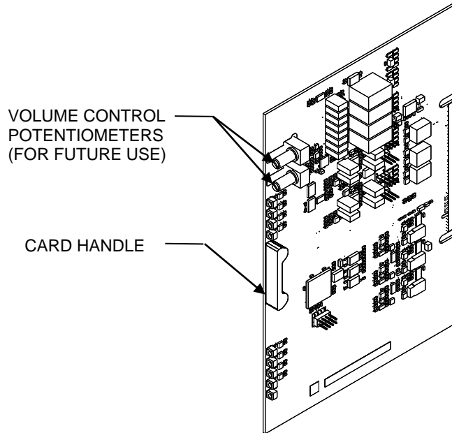
Figure 5 VCC2002-A1 Voice I/O Card Showing Handle and Volume Controls
