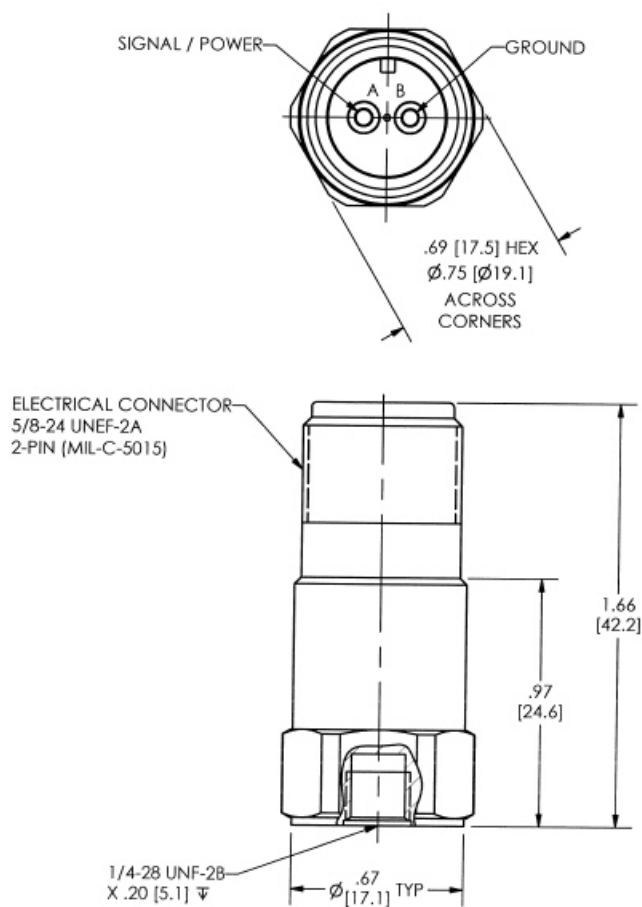
Figure 11 - 9300 Accelerometer Drawing
