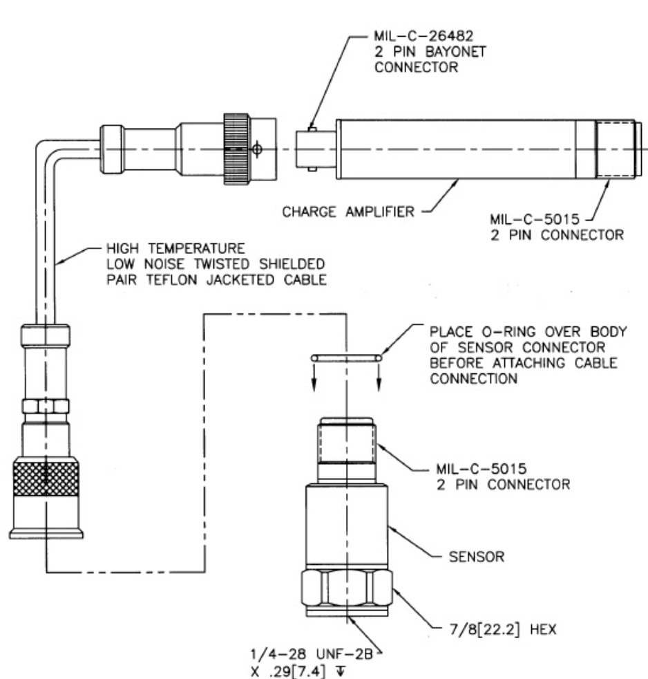
Figure 18 - 9150HT Accelerometer Drawing
