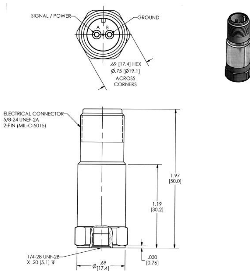
Figure 8 - 9010 Accelerometer Drawing
