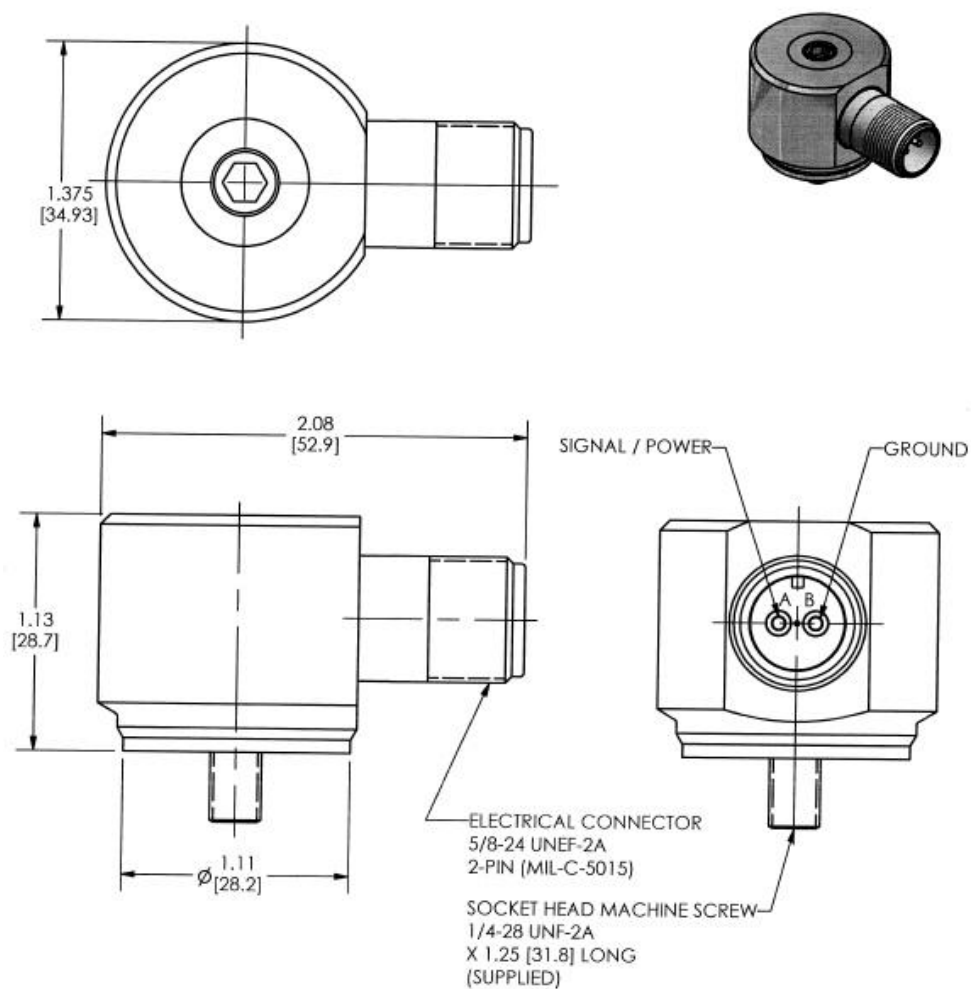
Figure 22 - 9200V0 Accelerometer Drawing
