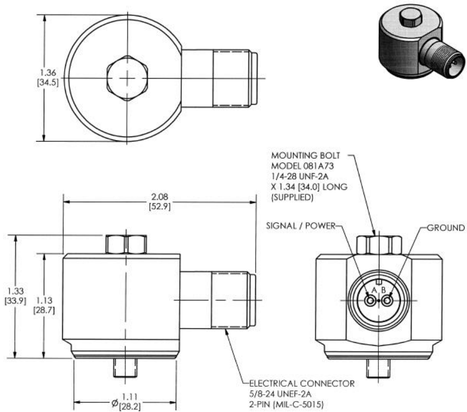
Figure 12 - 9400 Accelerometer Drawing
