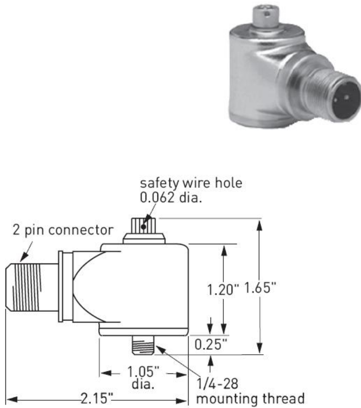
Figure 27 - 9200EX Accelerometer Drawing
