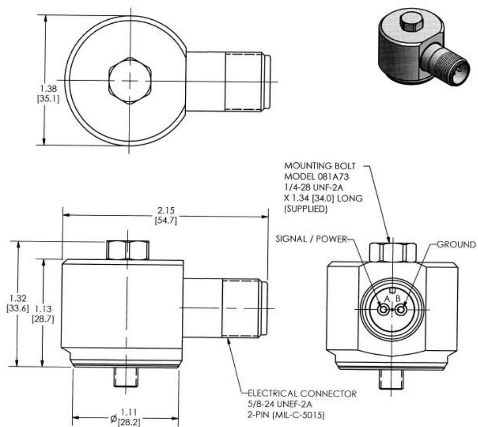
Figure 10 - 9200 Accelerometer Drawing
