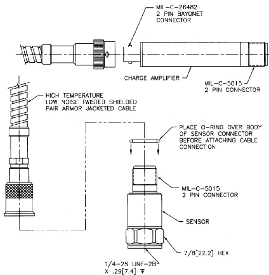
Figure 19 - 9150HTA Accelerometer Drawing
