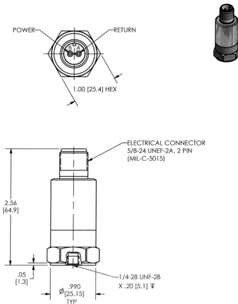
Figure 28 - 9842V Accelerometer Drawing
