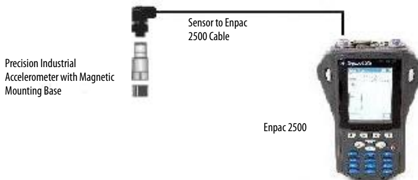
Figure 4 - Portable Data Collector and Accelerometer
