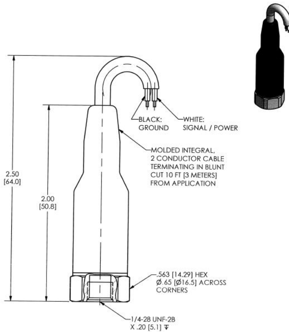
Figure 7 - 9008 Accelerometer Drawing
