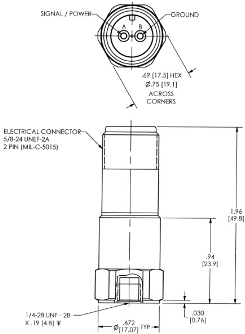
Figure 5 - 9000A Accelerometer Drawing
