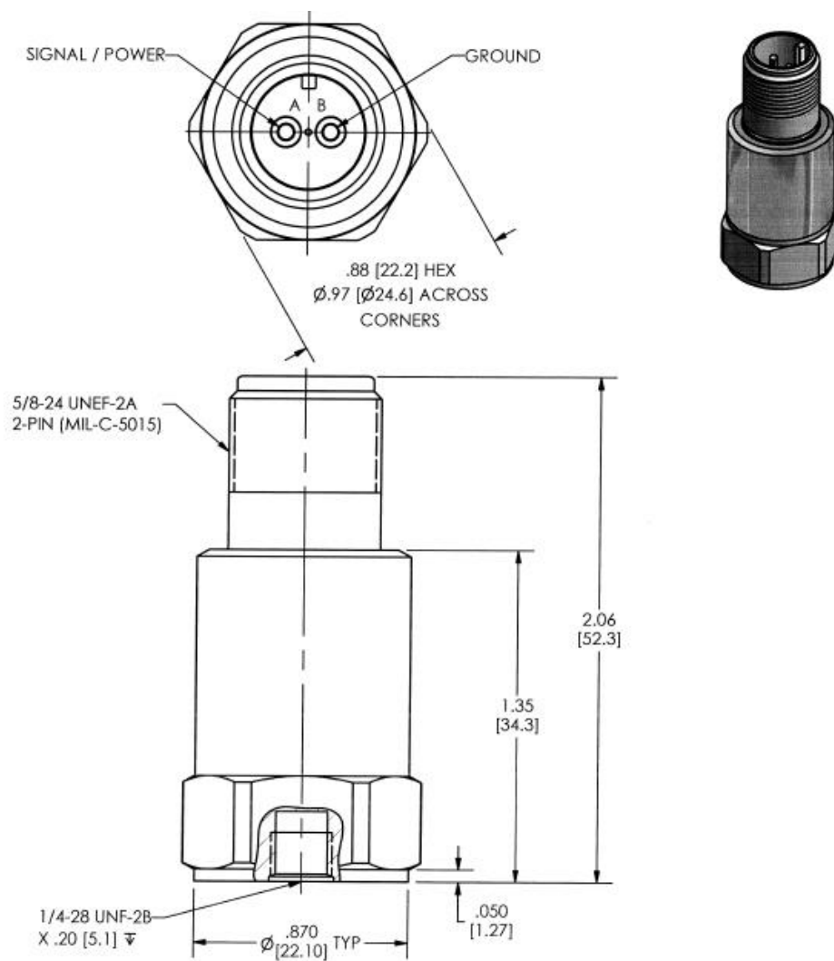
Figure 21 - 9100V0 Accelerometer Drawing
