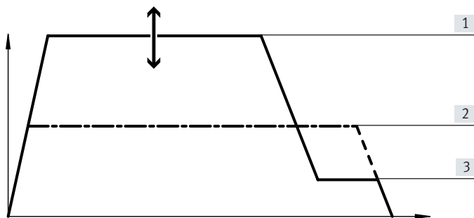
Y-axis: Cylinder speed X-axis: Cylinder stroke — A – Proportional valve - - - - B – Switching valve
