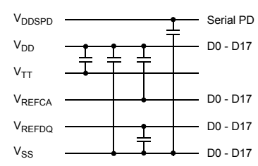
Serial PD w/integrated Thermal Sensor
