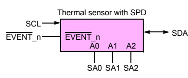
Serial PD w/integrated Thermal Sensor
