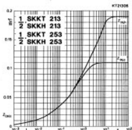
Fig. 6 Transient thermal impedance vs. time
